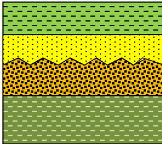
Gambar 5.10 disconformity
