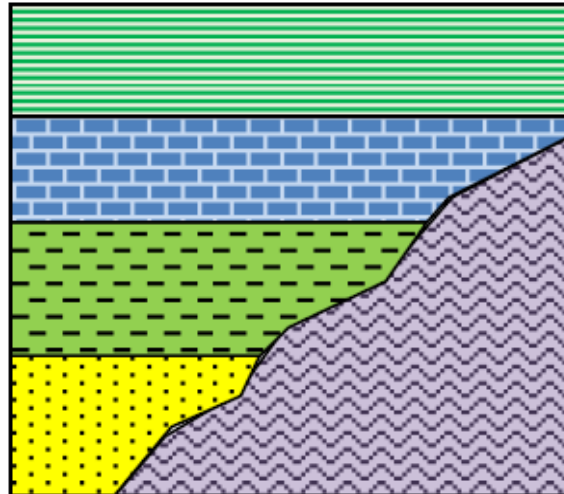
Gambar 5.12 nonconformity
