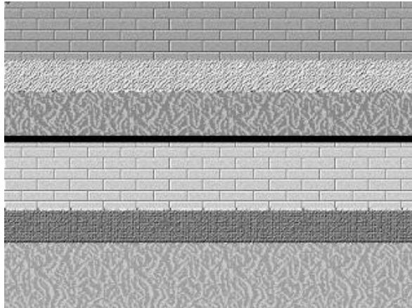
Gambar 5.11 paraconformity
