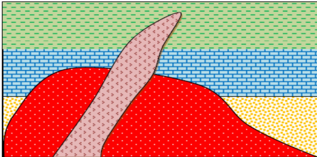
Gambar 5.7 Hukum cross cutting relationship
